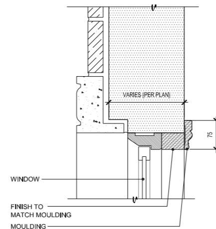
(A) HEAD JAMB SECTION
