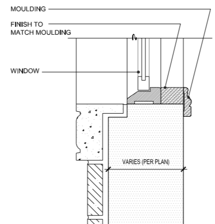
(C) SILL SECTION
