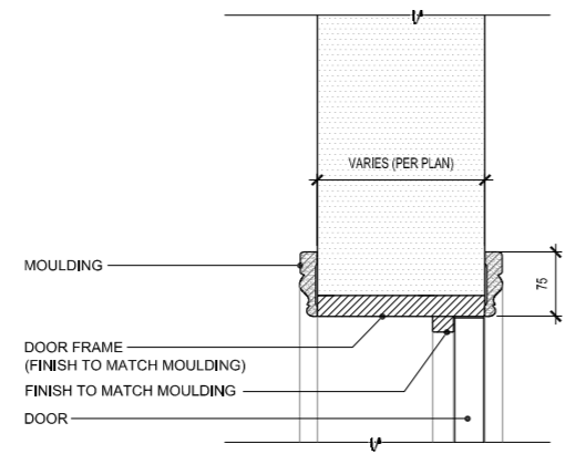
(A) HEAD JAMB SECTION
